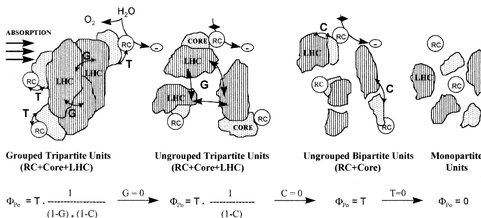
Fig. 9. Alteration in the architecture of PSII units after heat treatment and their effect on the maximum quantum yield for primary photochemistry, \Phi_{P_0} . Monopartite units correspond to pigment protein complexes which are totally disconnected from the RC. ♦ indicates the block in electron donation from the oxygen evolving complex. Core antenna complexes are shaded with dots and LHC complexes are shaded with vertical lines.
