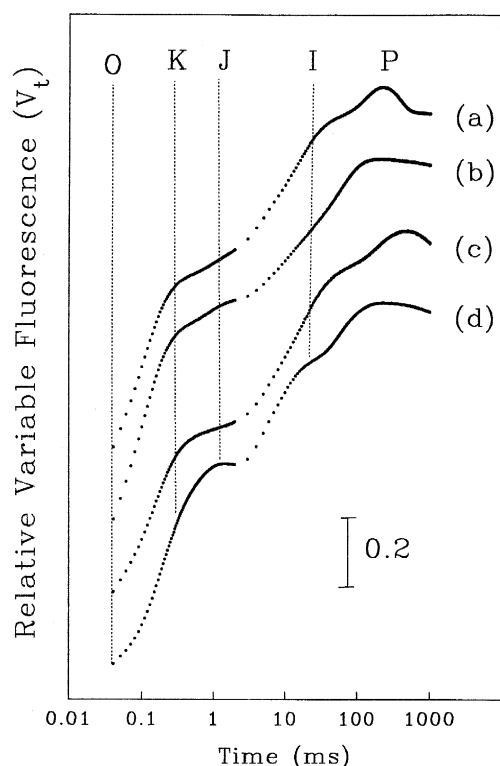
Fig. 7. Relative variable Chl a fluorescence ( V_t = (F_t - F_0)/(F_m - F_0) ) of leaves of Permelia sp. (a), Cycus revoluta (b) and the fruits of Juniperus sp. (c). Measurements were done directly on the sample in the field after 1 h of dark adaptation. All the traces show the existence of a K-step. For comparison, curve (d) has been plotted which has been measured from a pea leaf, grown in the green house, displays only O-J-I-P steps of the Chl a fluorescence transient.
