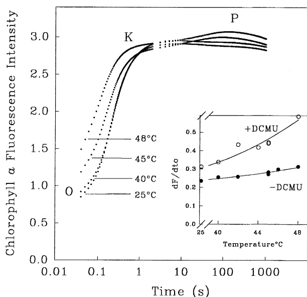
Fig. 5. Effect of DCMU (250 \mu M) and heat treatment on Chl a fluorescence transients of pea leaf discs. After the heat stress at different temperatures for 5 min, the leaf discs were kept in incubation medium with 250 \mu M DCMU for 2 h in complete darkness at room temperature. Insert shows the changes in the Chl a fluorescence intensity from 40 \mu s up to 100 \mu s in the presence or absence of DCMU at different temperatures. The addition of NH_2OH to the heat treated sample in the presence of DCMU did not change the shape of the curves (not shown in this figure).
