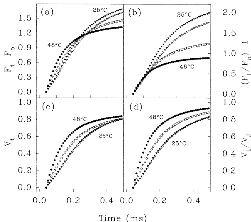
Fig. 6. a: the fast rise of the variable fluorescence ( F_t - F_0 ) without any normalization during the first 0.5 ms after heat treatment for 5 min at 25 ( \Delta ), 40 ( \blacktriangle ), 46 ( \circ ) and 48 ( \bullet ) °C and incubation for 2 h in DCMU at room temperature. b: same data as in (a) but normalized to the initial fluorescence intensity, F_0 . c: the relative variable fluorescence, V_t = (F_t - F_0)/(F_m - F_0) . d: the variable fluorescence ( F_t - F_0 ) normalized by the variable fluorescence at 2 ms, V_t/V_J = F_t/(F_{2\text{ ms}} - F_0) . The slope at the origin in the presence of DCMU is a measure of the maximum fractional rate of primary photochemistry, (dQ_A^-/Q_{A(\text{total})})/dt_0 , according to Eq. (7). The expression V_t/V_J without DCMU substitutes the expression V_t in presence of DCMU [56,57].
