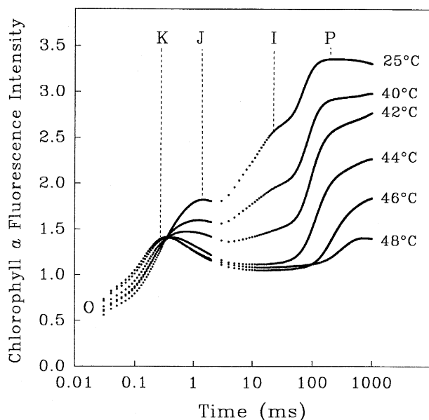
Fig. 1. Temperature dependence of the appearance of the K-step. Pea leaf discs were heated at the indicated temperatures for 5 min and readapted at room temperature for 10 s before the measurements. These are the original data, as measured, without any normalization.
