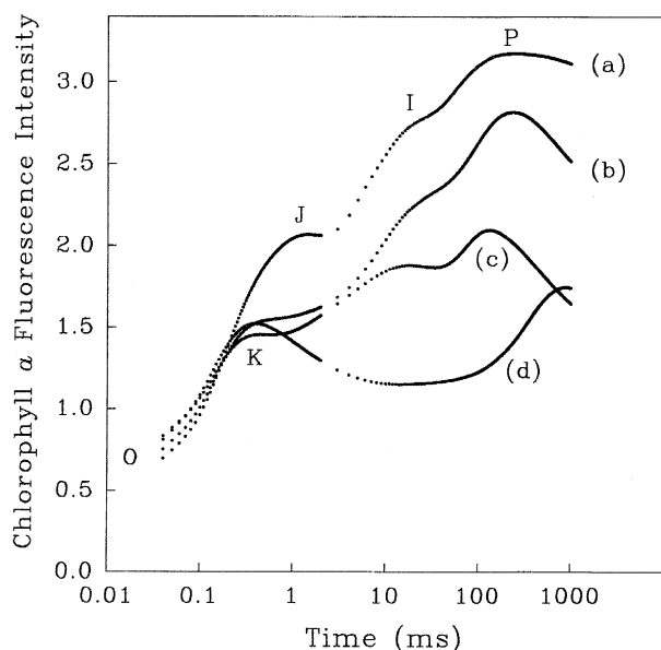
Fig. 4. Effect of NH_2OH on Chl a fluorescence transients of heat stressed pea leaf discs. a: control and (d) heat stress (5 min at 46°C) leaf discs kept in incubation medium for 2 h at room temperature; b: control and (c) heat stress (5 min at 46°C) leaf discs kept in incubation medium with 50 mM NH_2OH for 2 h at room temperature.
