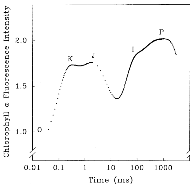
Fig. 2. Chlorophyll a fluorescence transients of a pea leaf disc after heat treatment (13 min at 44°C) and dark adaptation at room temperature for 10 s. The graph plotted on logarithmic time scale distinctly shows the K, J, I steps in between O and P.
