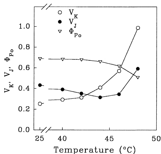
Fig. 3. Effect of temperature on the maximum quantum yield of excitation energy trapping ( \Phi_{P0} ) the relative variable fluorescence at the J-step ( V_J ), and the K-step ( V_K ) of pea leaves. \Phi_{P0} was measured in presence of DCMU.
