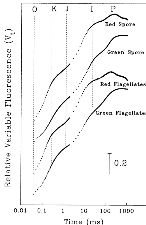
Fig. 8. Relative variable Chl a fluorescence ( V_t = (F_t - F_0)/(F_m - F_0) ) of dark adapted green or red flagellates of Haematococcus lacustris and its red or green spores. A clear K-step is visible in red spores and red flagellates.
